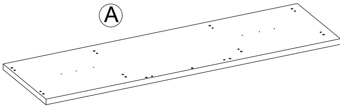
TOP SHELF T1822920010GO QTY: 1 PC
